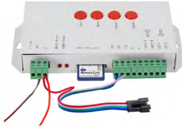
DIGITAL LED STRIP CONTROLLER DC5-24V SD-CARD
